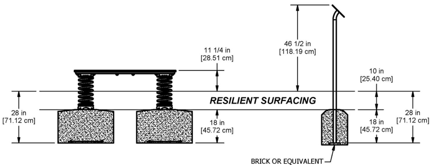
ELEVATION VIEW
