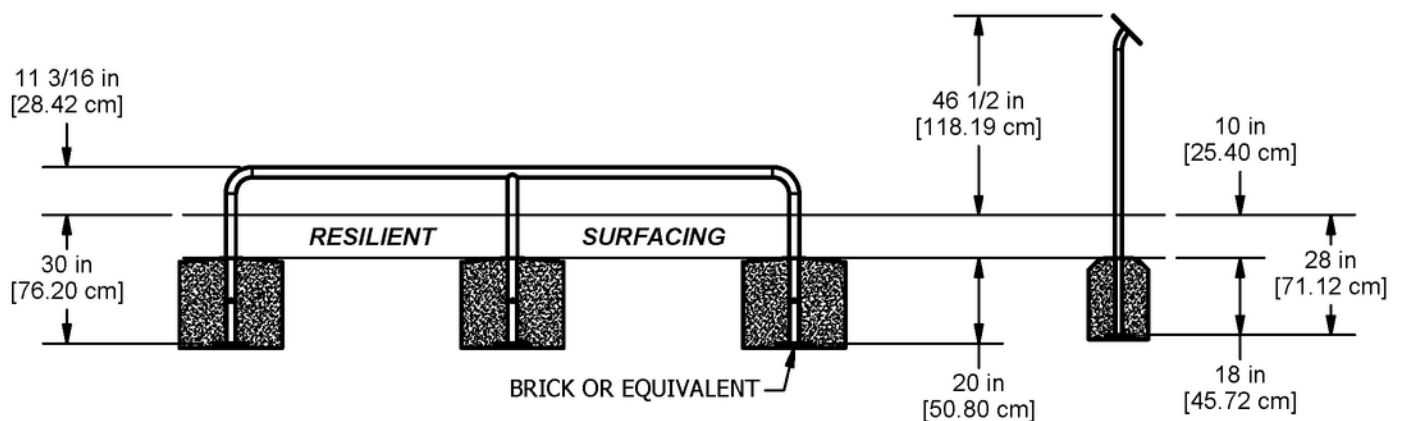
ELEVATION VIEW
