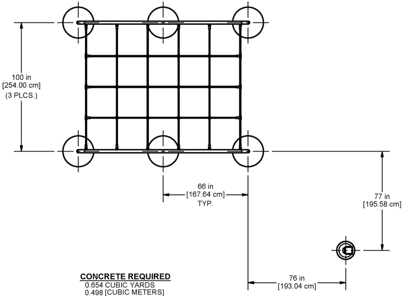
PLAN VIEW
